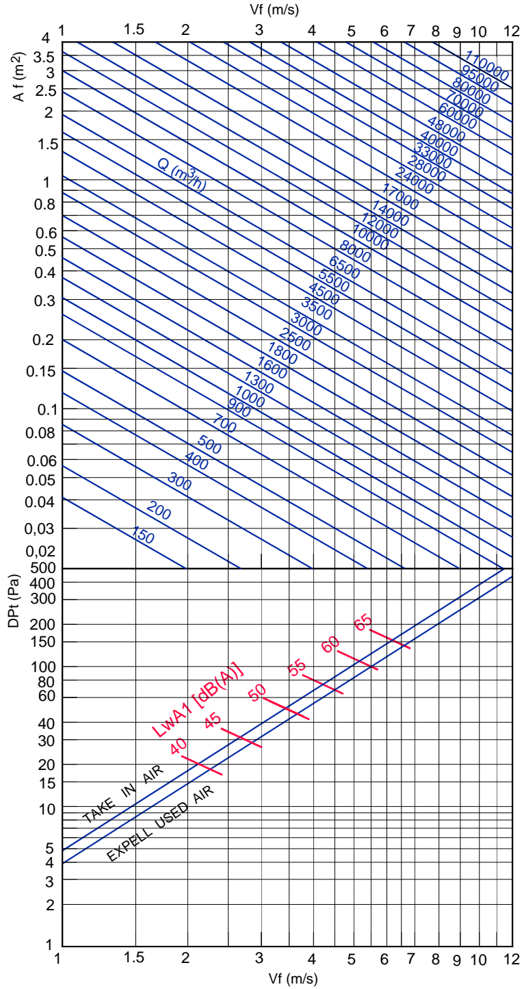
FREE VELOCITY, PRESSURE LOSS AND SOUND POWER LEVEL.
