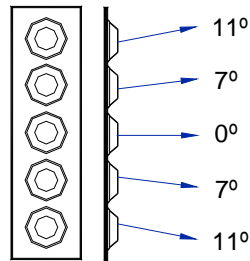
POSITION 2 (22°)
