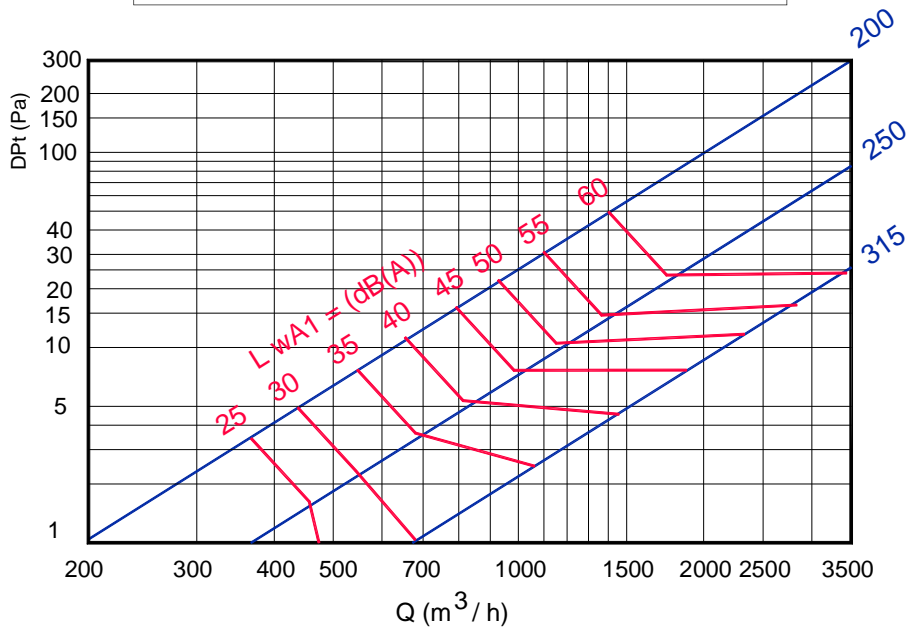
PRESSURE DROP AND SOUND POWER LEVEL
